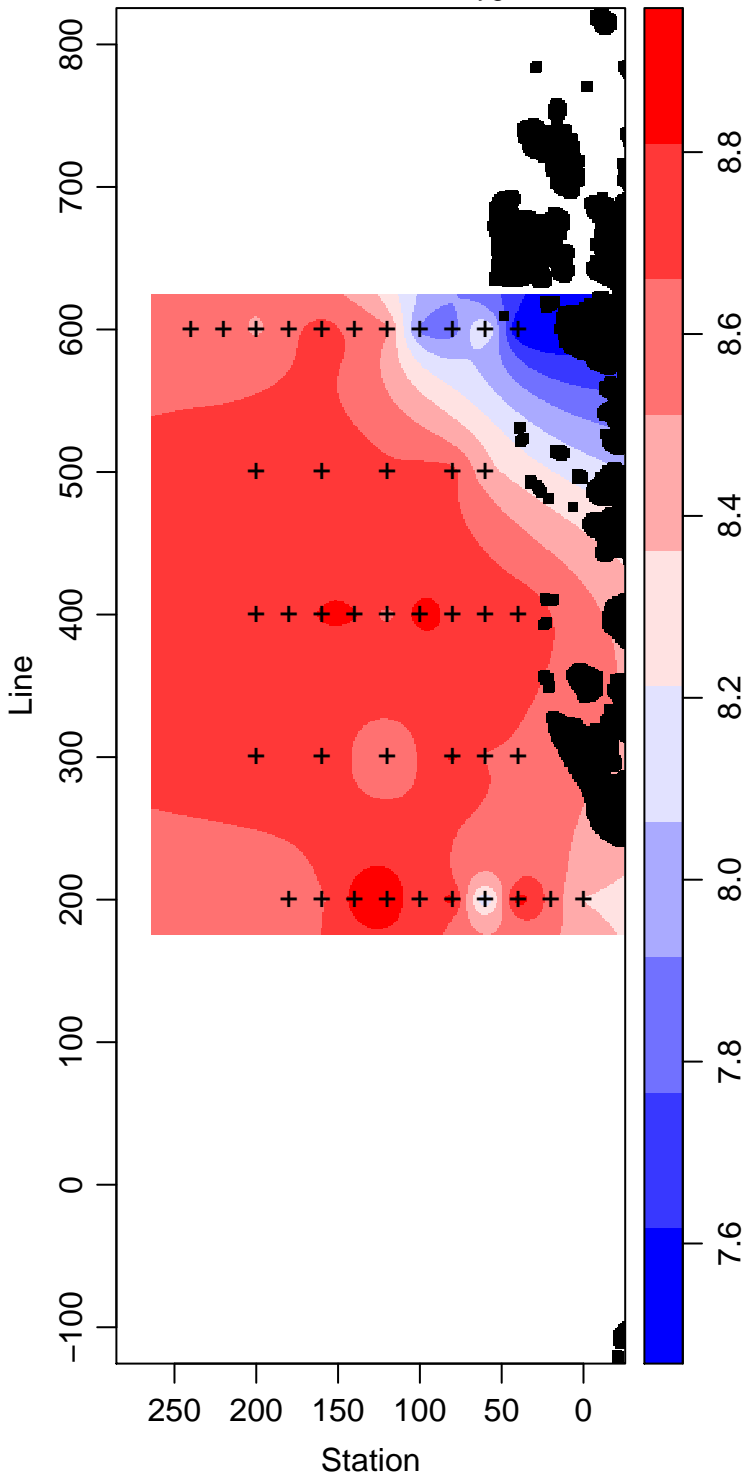
LMG00-01_30_Dissolved.Oxygen ml L -1
