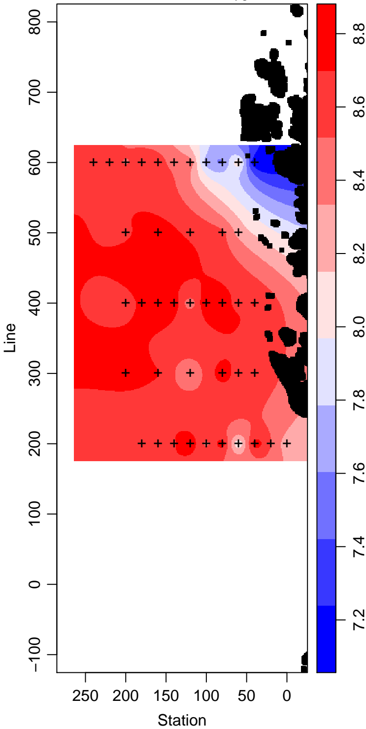
LMG00-01_35_Dissolved.Oxygen ml L -1
