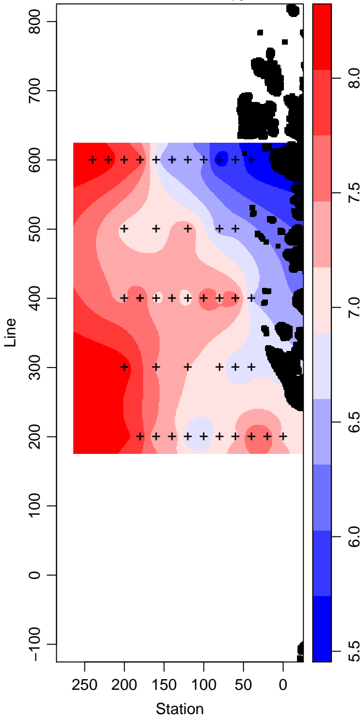
LMG00-01_80_Dissolved.Oxygen ml L -1
