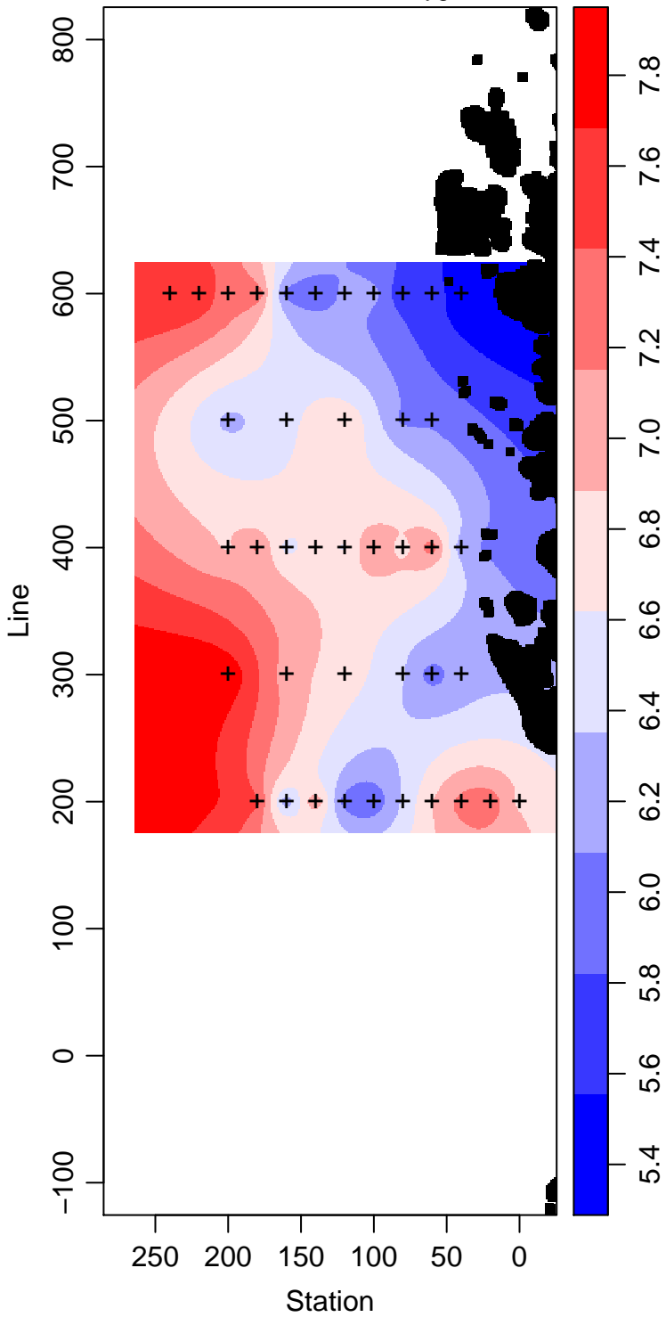
LMG00-01_95_Dissolved.Oxygen ml L -1
