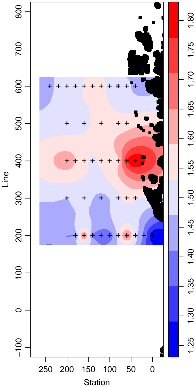
LMG00-01_10_Phosphate \mu\text{ mol L}^{-1}
