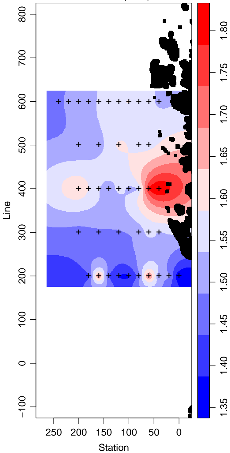
LMG00-01_15_Phosphate \mu\text{ mol L}^{-1}
