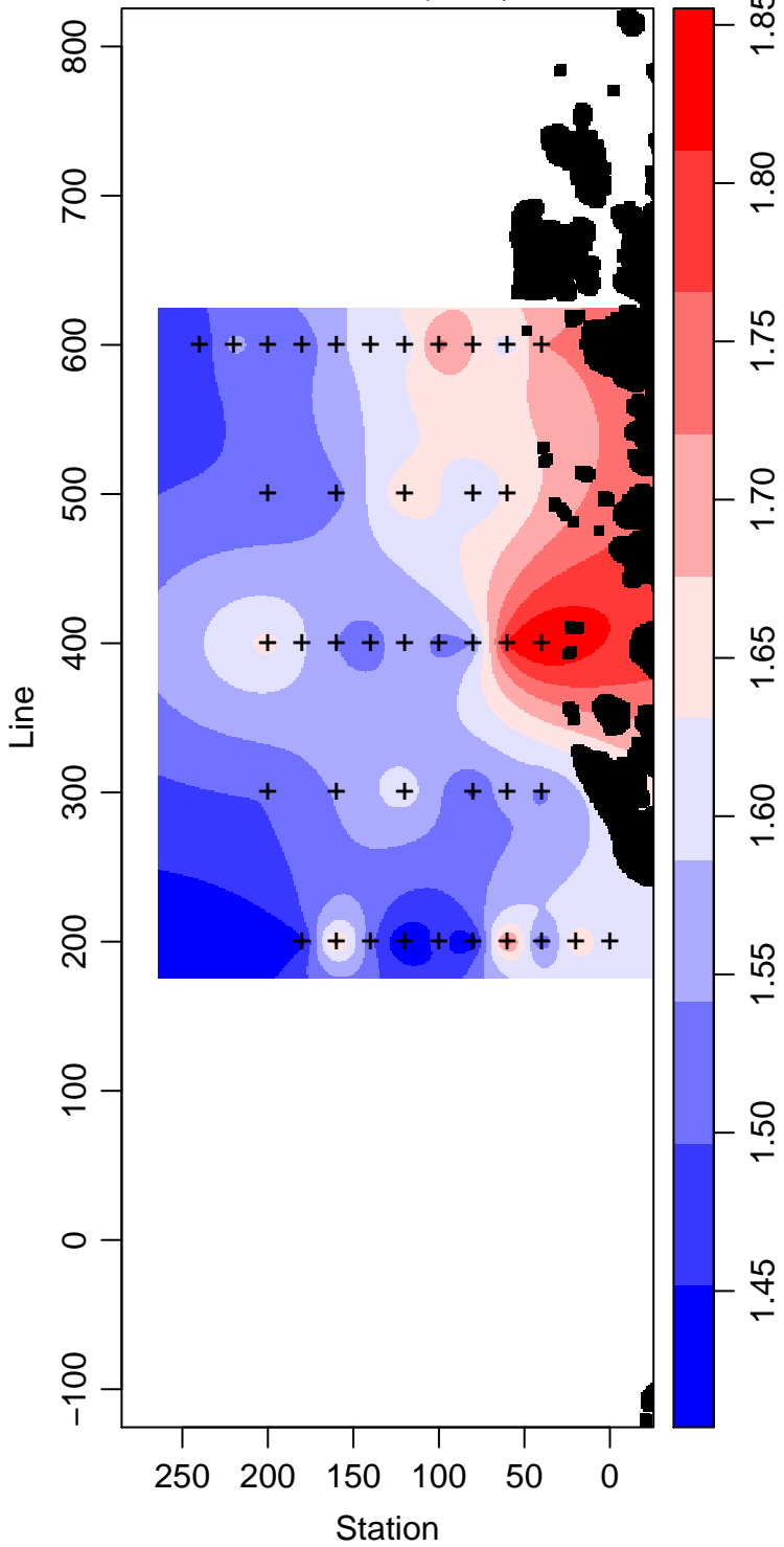
LMG00-01_25_Phosphate \mu\text{ mol L}^{-1}
