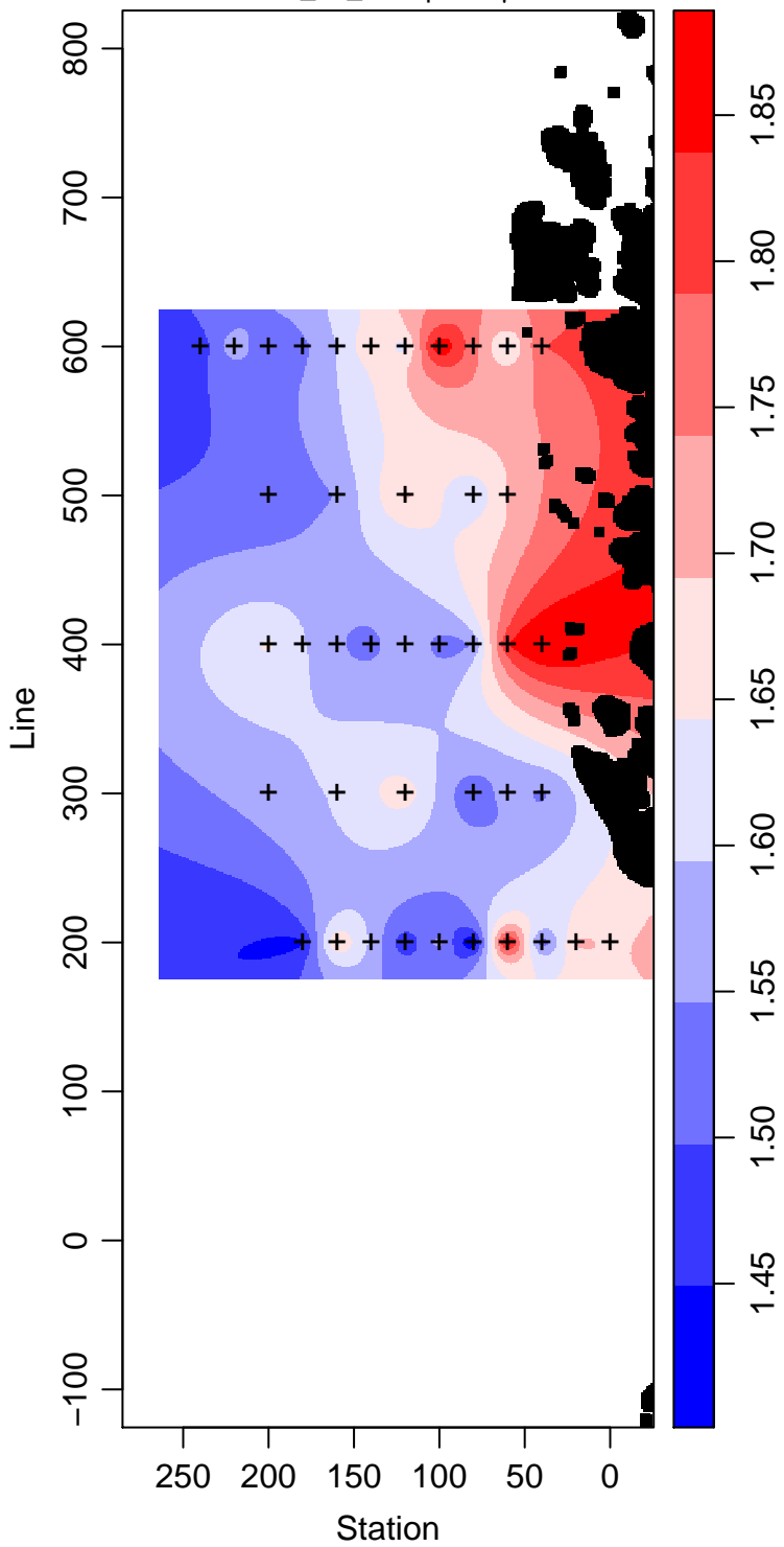
LMG00-01_30_Phosphate \mu\text{ mol L}^{-1}
