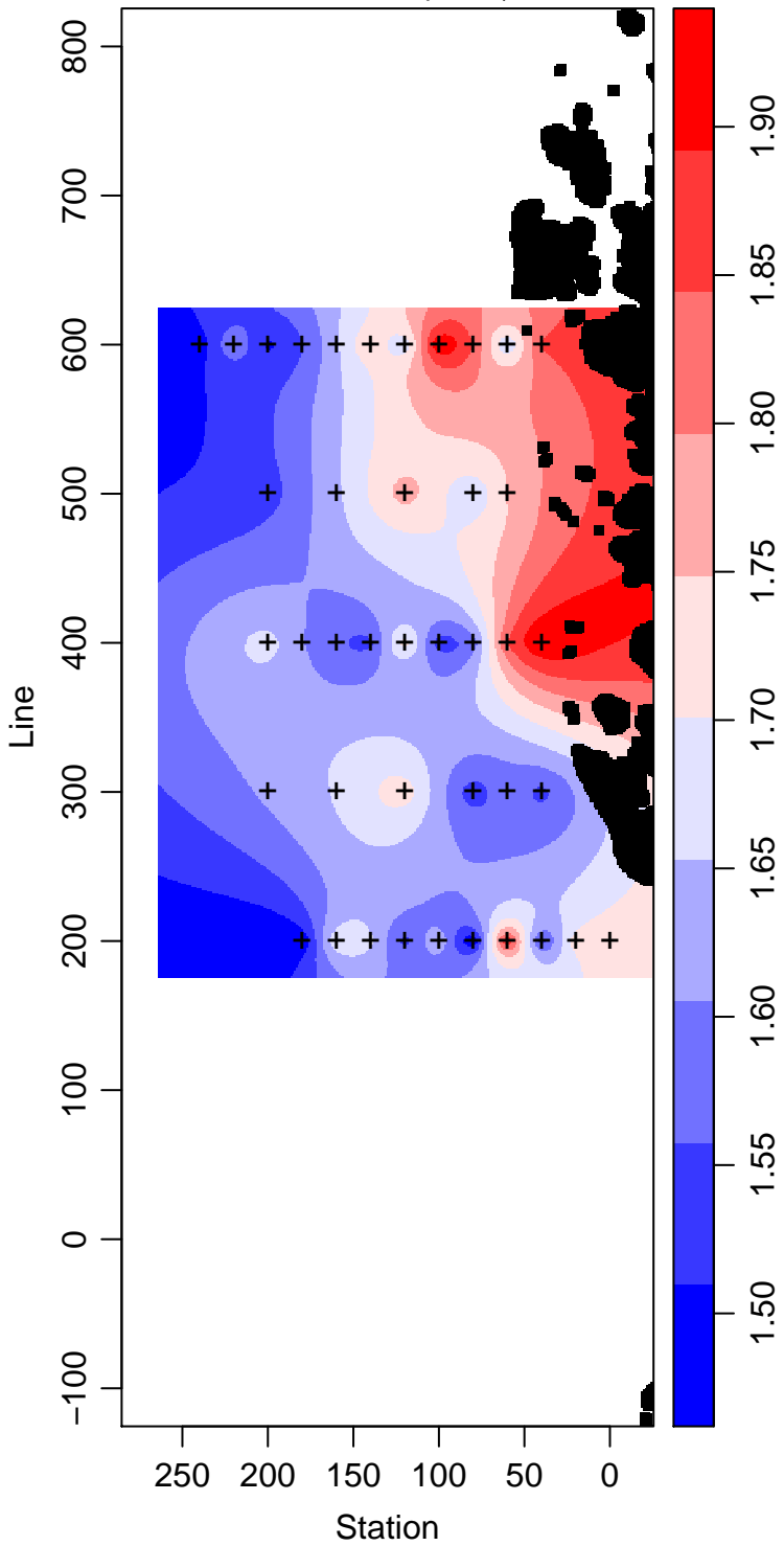
LMG00-01_35_Phosphate \mu\text{ mol L}^{-1}
