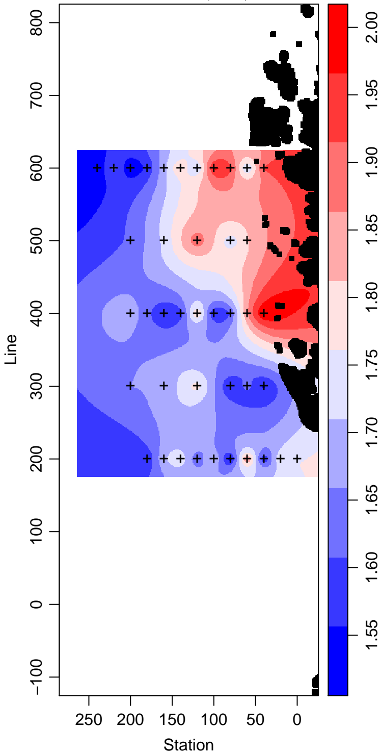
LMG00-01_40_Phosphate \mu\text{ mol L}^{-1}
