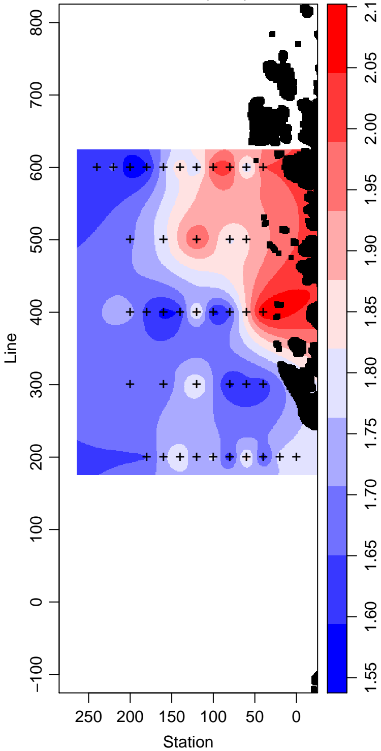
LMG00-01_45_Phosphate \mu\text{ mol L}^{-1}
