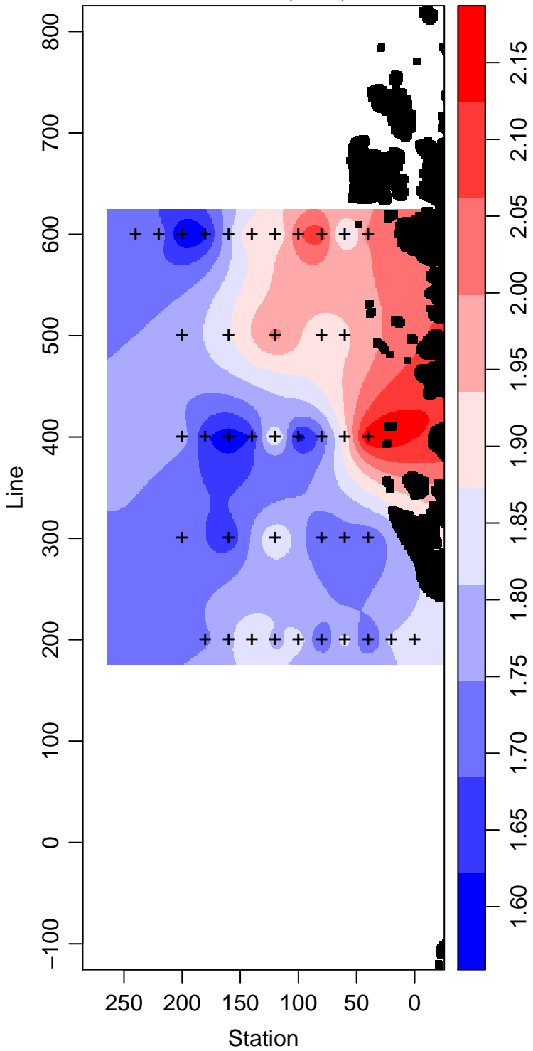
LMG00-01_50_Phosphate \mu\text{ mol L}^{-1}
