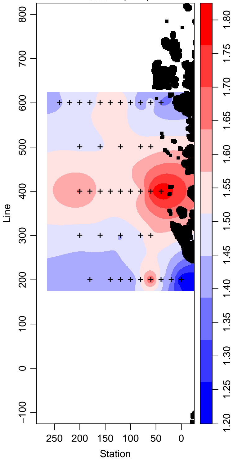
LMG00-01_5_Phosphate \mu\text{ mol L}^{-1}
