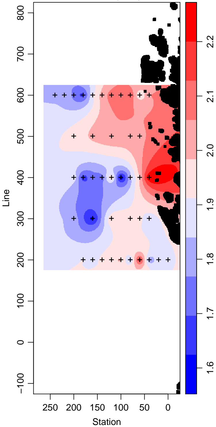
LMG00-01_60_Phosphate \mu\text{ mol L}^{-1}
