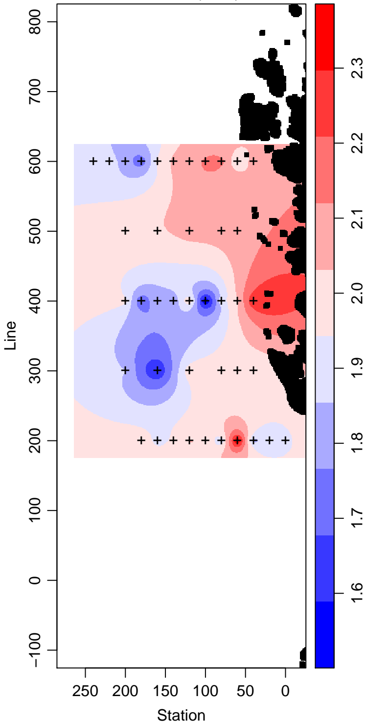
LMG00-01_65_Phosphate \mu\text{ mol L}^{-1}
