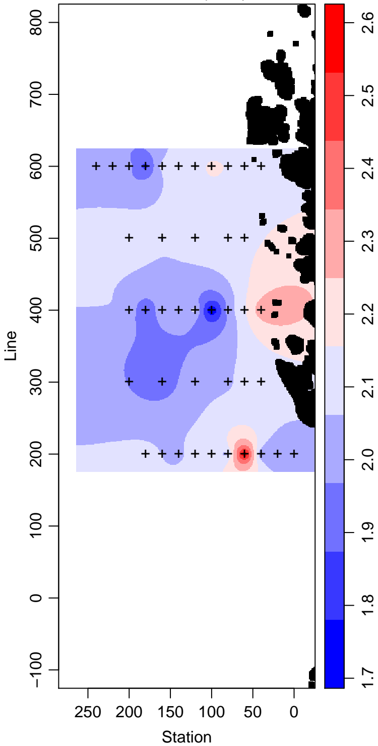
LMG00-01_80_Phosphate \mu\text{ mol L}^{-1}
