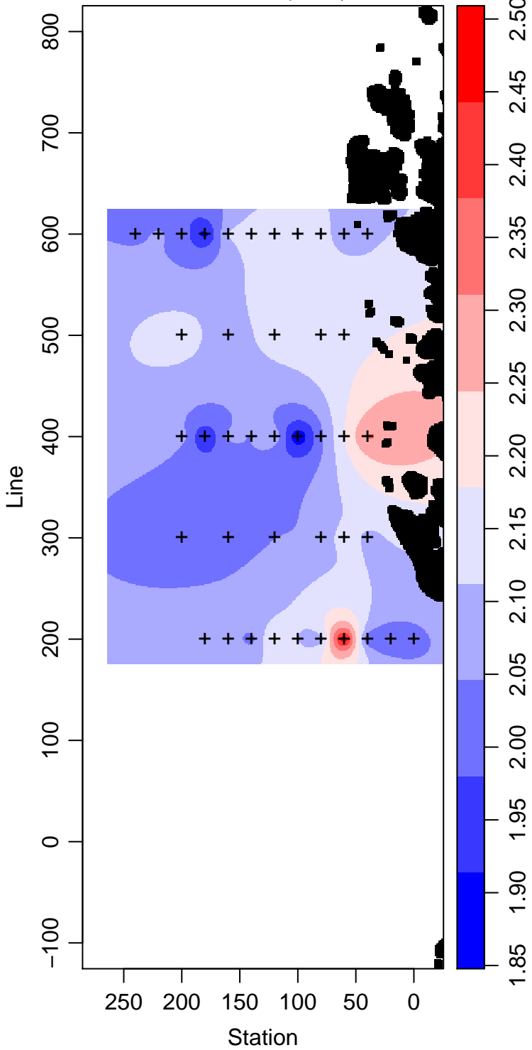
LMG00-01_85_Phosphate \mu\text{ mol L}^{-1}
