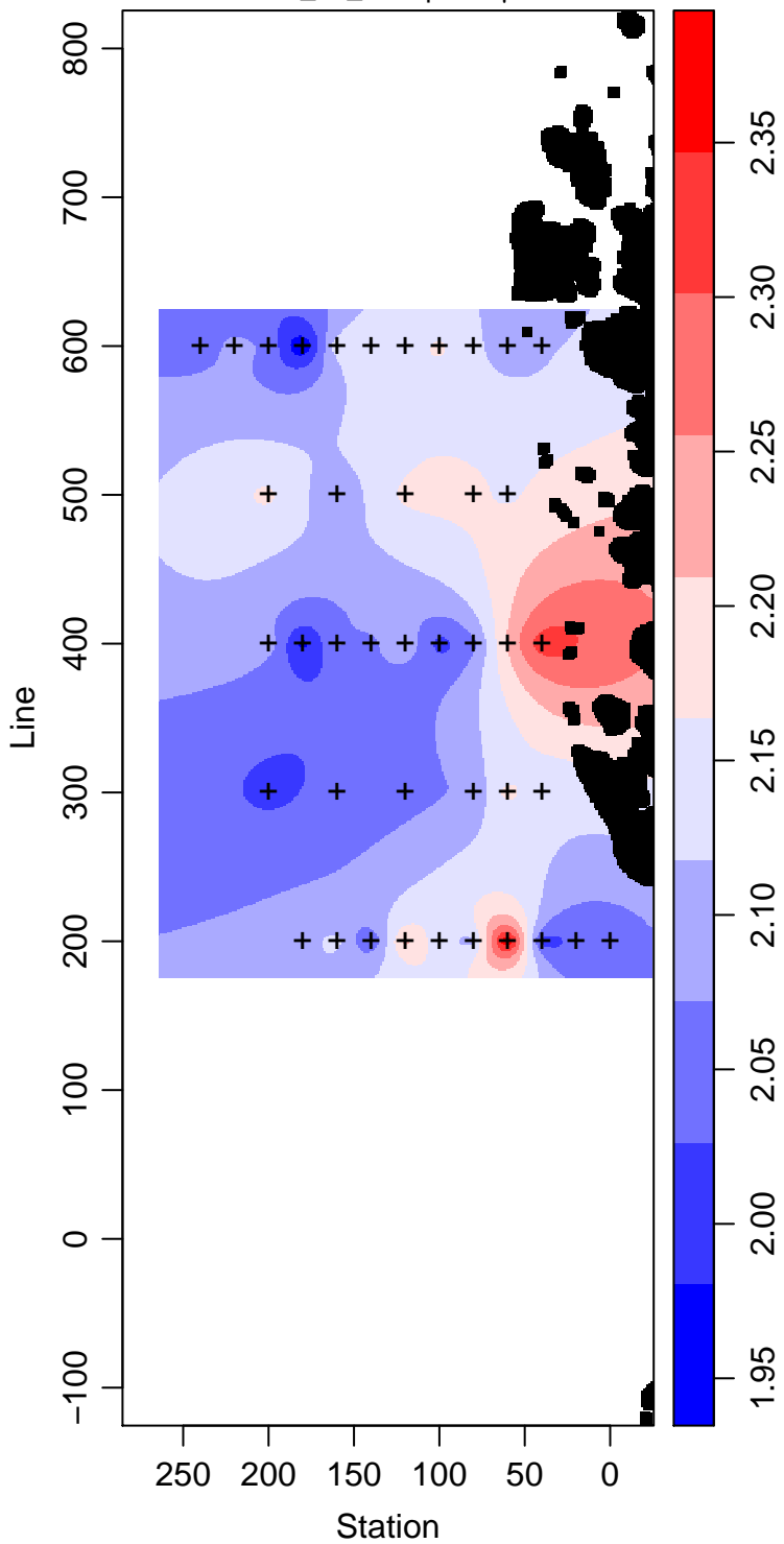
LMG00-01_90_Phosphate \mu\text{ mol L}^{-1}
