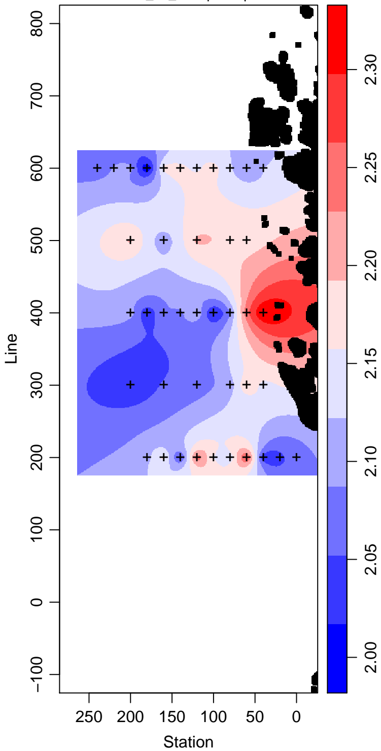
LMG00-01_95_Phosphate \mu\text{ mol L}^{-1}
