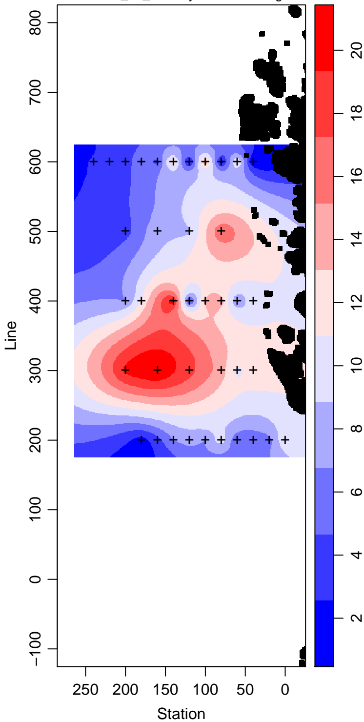
LMG00-01_25_Primary.Production mg m -3
