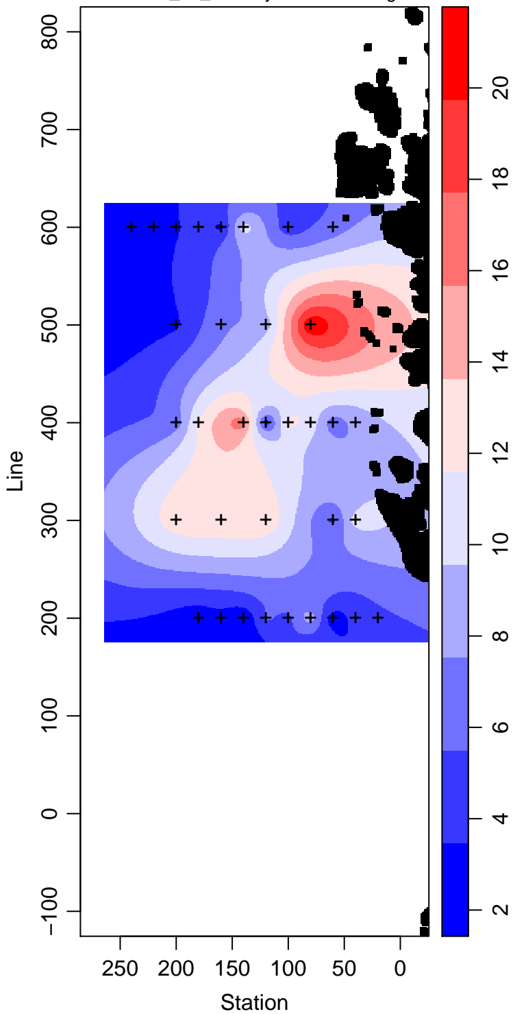
LMG00-01_30_Primary.Production mg m -3
