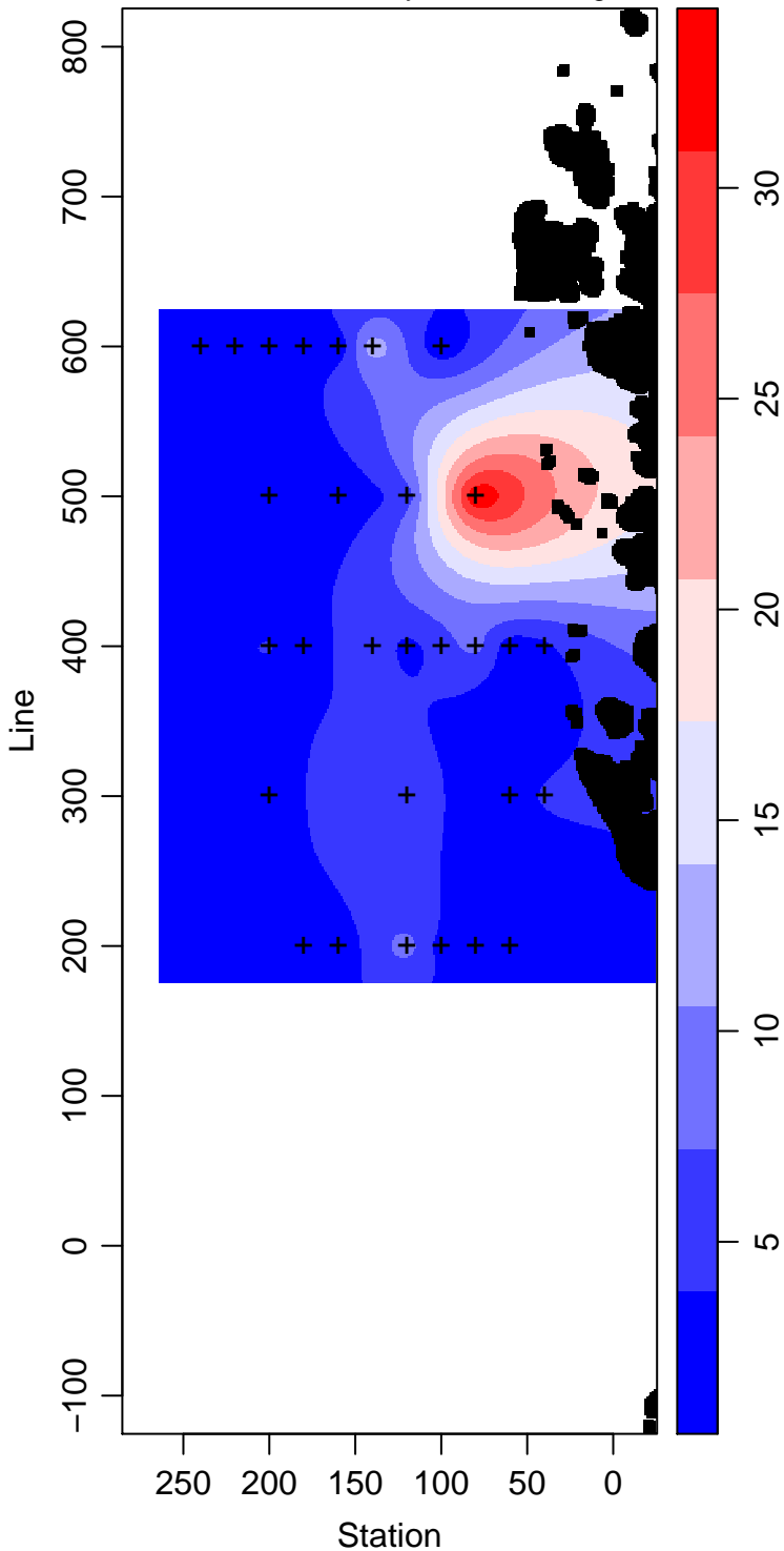
LMG00-01_45_Primary.Production mg m -3
