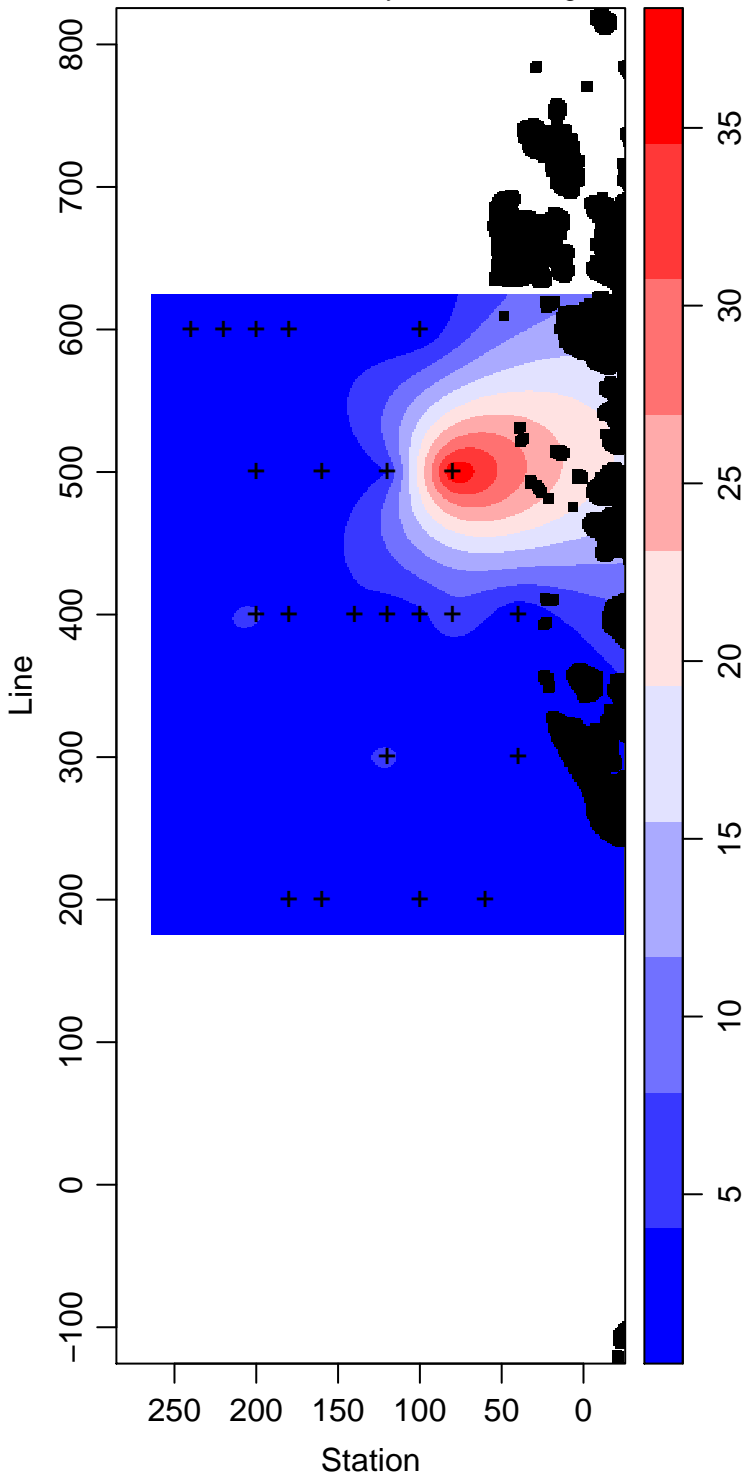
LMG00-01_50_Primary.Production mg m -3
