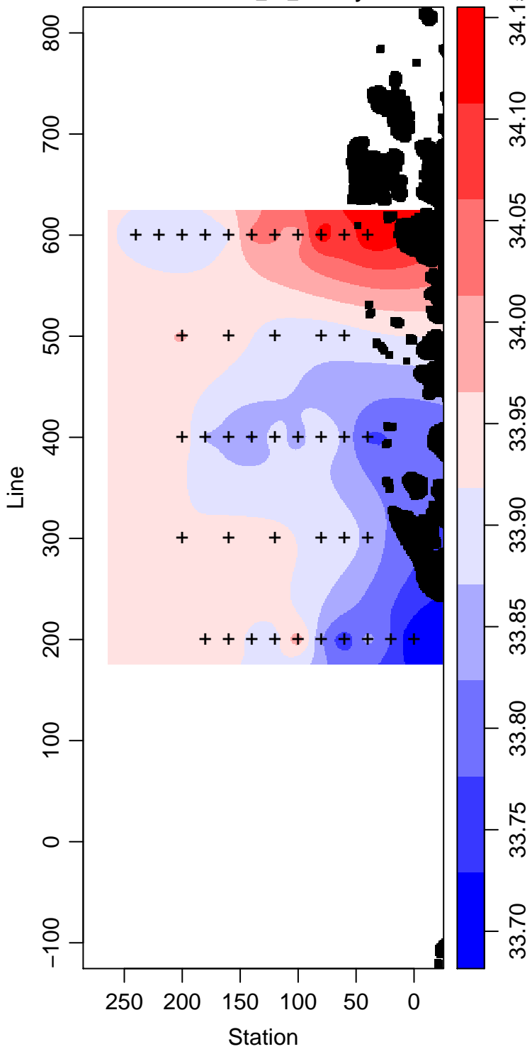
LMG00-01_55_Salinity
