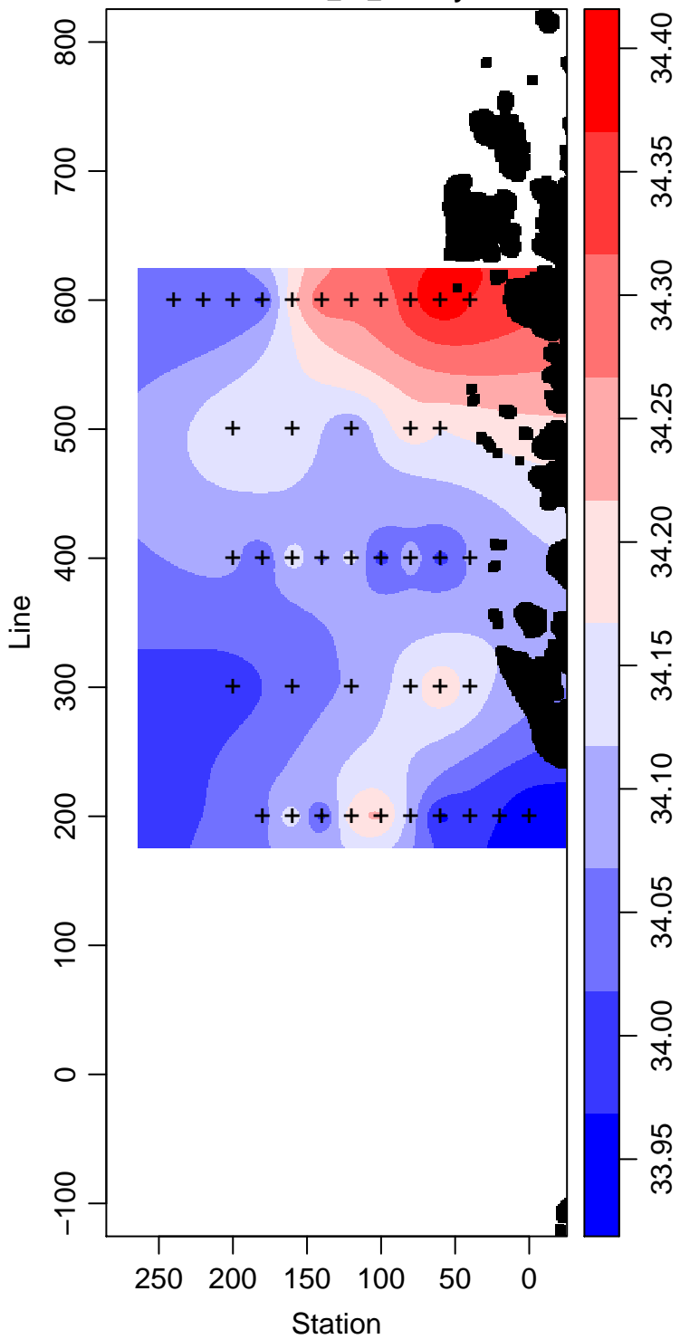
LMG00-01_85_Salinity
