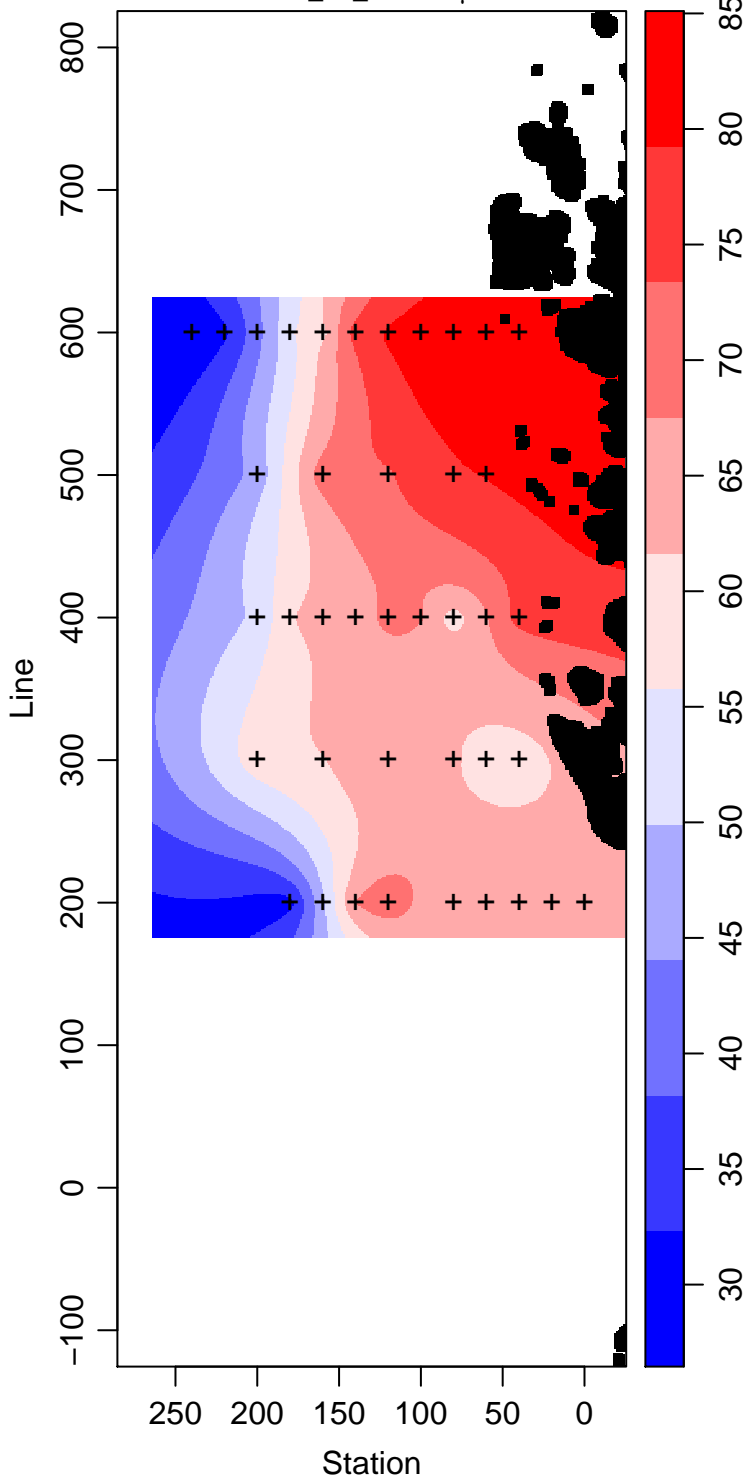
LMG00-01_15_Silicate \mu\text{ mol L}^{-1}
