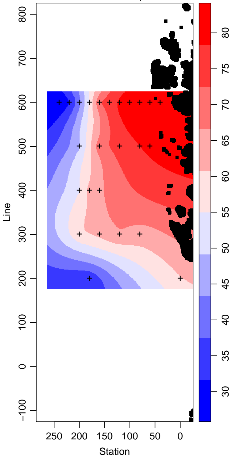
LMG00-01_1_Silicate \mu\text{ mol L}^{-1}
