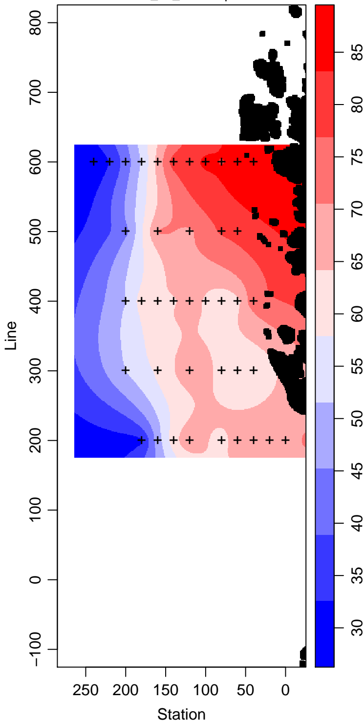
LMG00-01_30_Silicate \mu\text{ mol L}^{-1}
