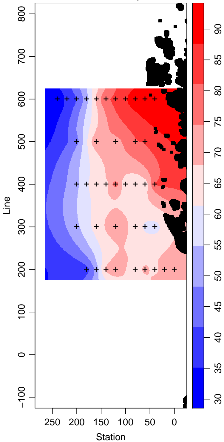
LMG00-01_45_Silicate \mu\text{ mol L}^{-1}
