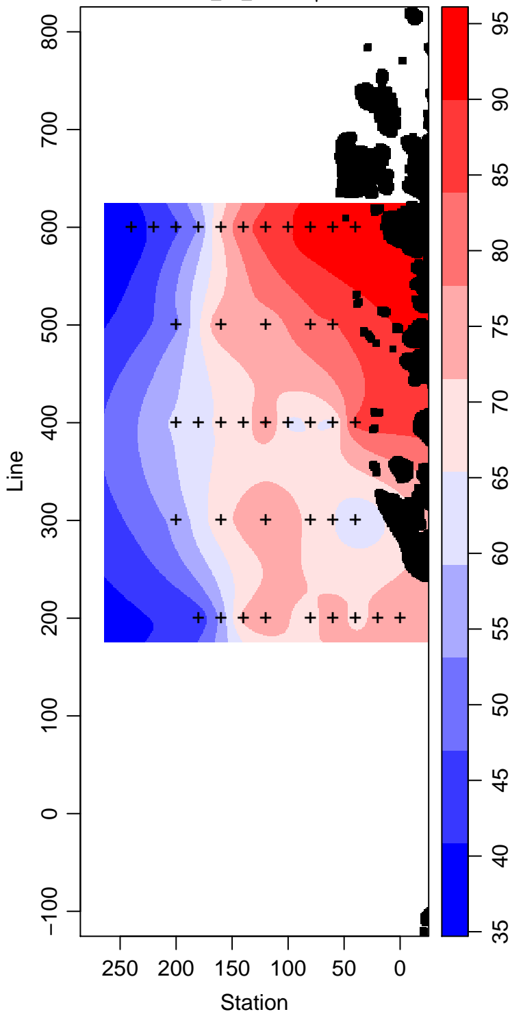
LMG00-01_55_Silicate \mu\text{ mol L}^{-1}
