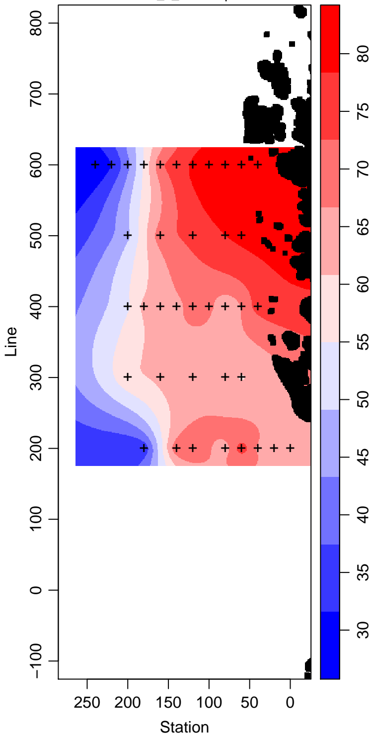
LMG00-01_5_Silicate \mu\text{ mol L}^{-1}
