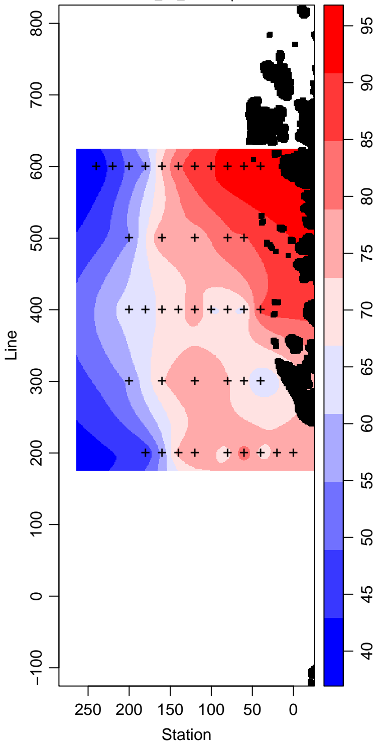
LMG00-01_60_Silicate \mu\text{ mol L}^{-1}
