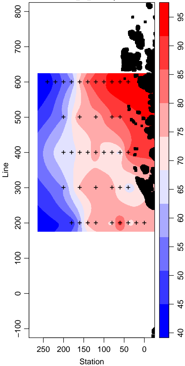
LMG00-01_65_Silicate \mu\text{ mol L}^{-1}
