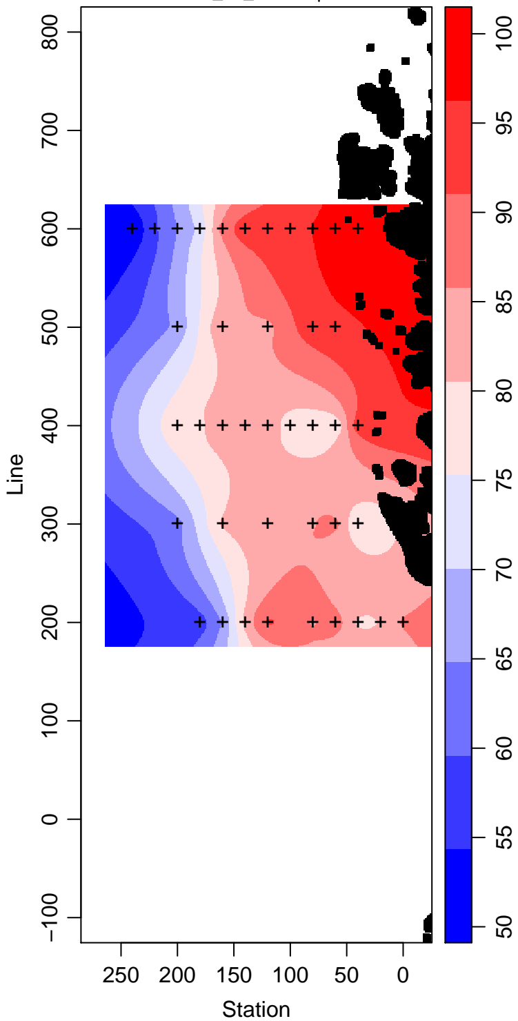
LMG00-01_95_Silicate \mu\text{ mol L}^{-1}
