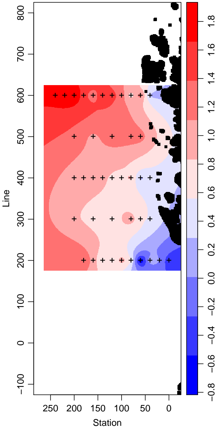
LMG00-01_15_Temperature ° Celsius
