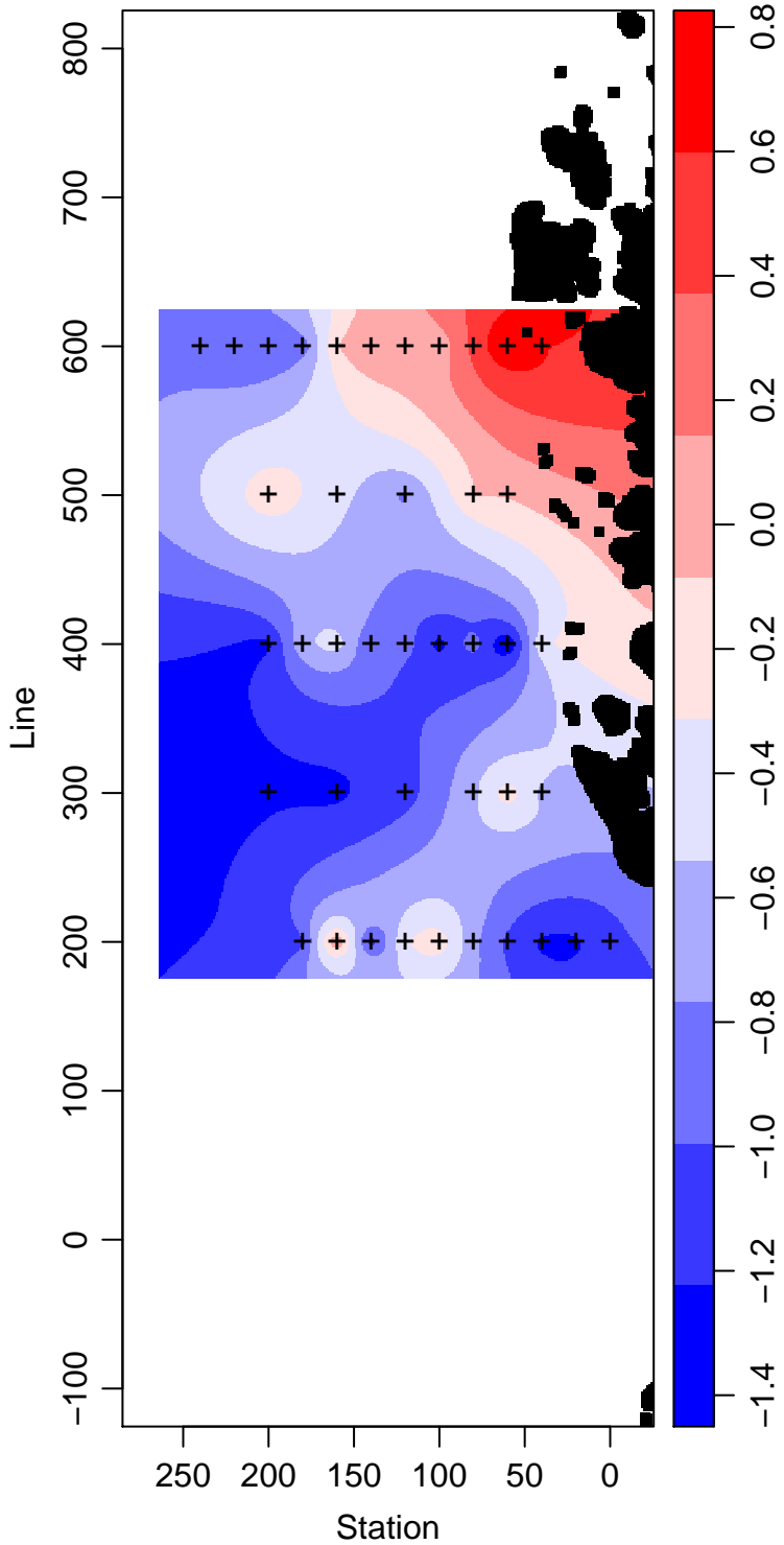
LMG00-01_95_Temperature ° Celsius
