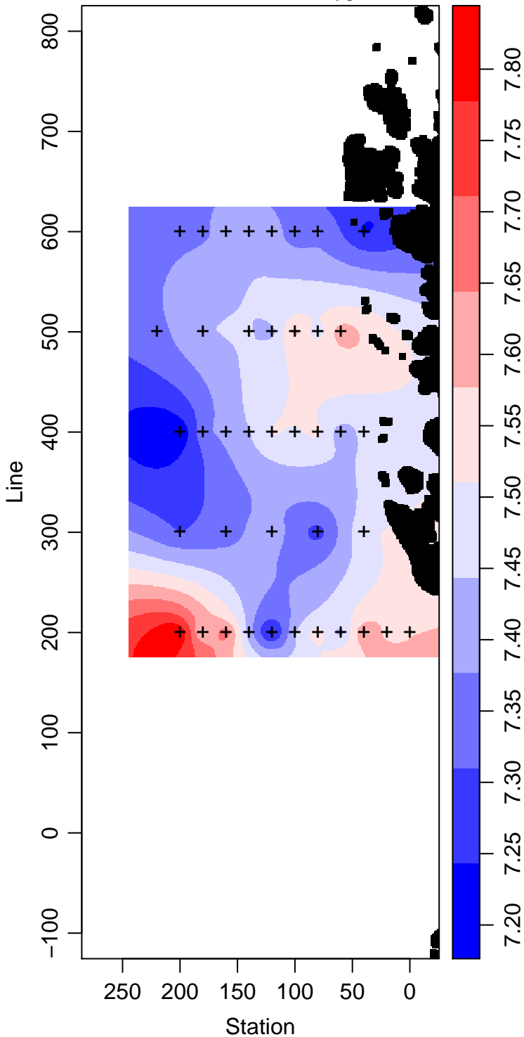
LMG01-01_35_Dissolved.Oxygen ml L -1
