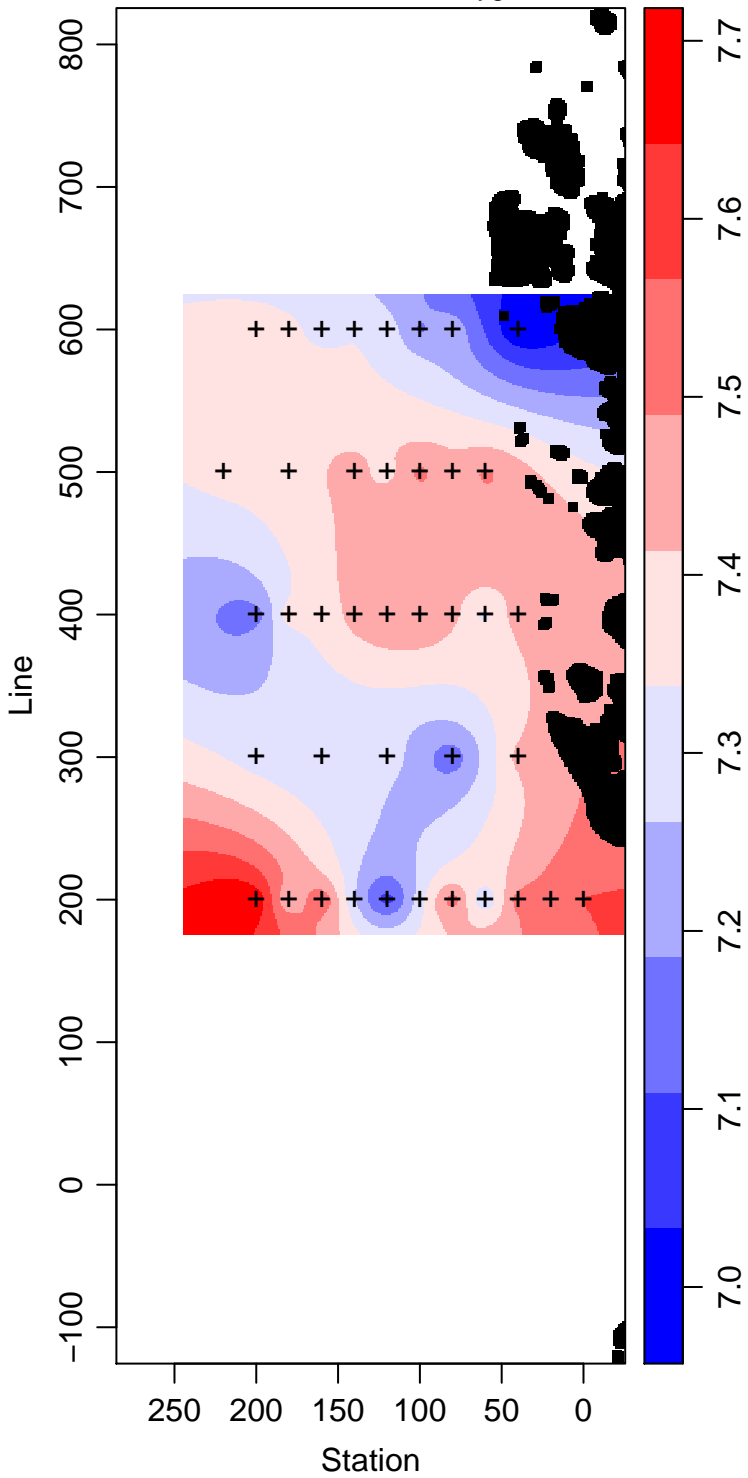
LMG01-01_40_Dissolved.Oxygen ml L -1
