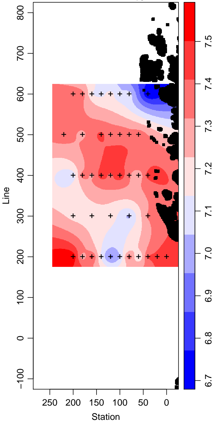
LMG01-01_45_Dissolved.Oxygen ml L -1
