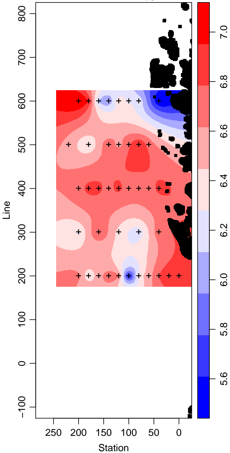
LMG01-01_75_Dissolved.Oxygen ml L -1
