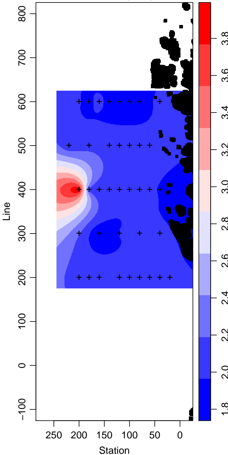
LMG01-01_100_Phosphate \mu\text{ mol L}^{-1}
