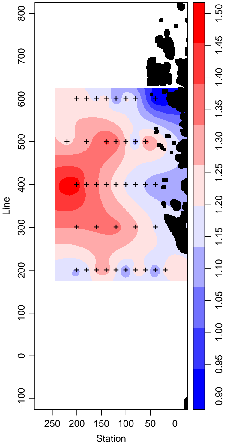
LMG01-01_10_Phosphate \mu\text{ mol L}^{-1}
