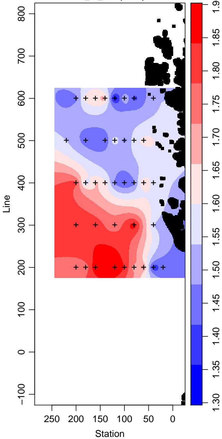
LMG01-01_50_Phosphate \mu\text{ mol L}^{-1}
