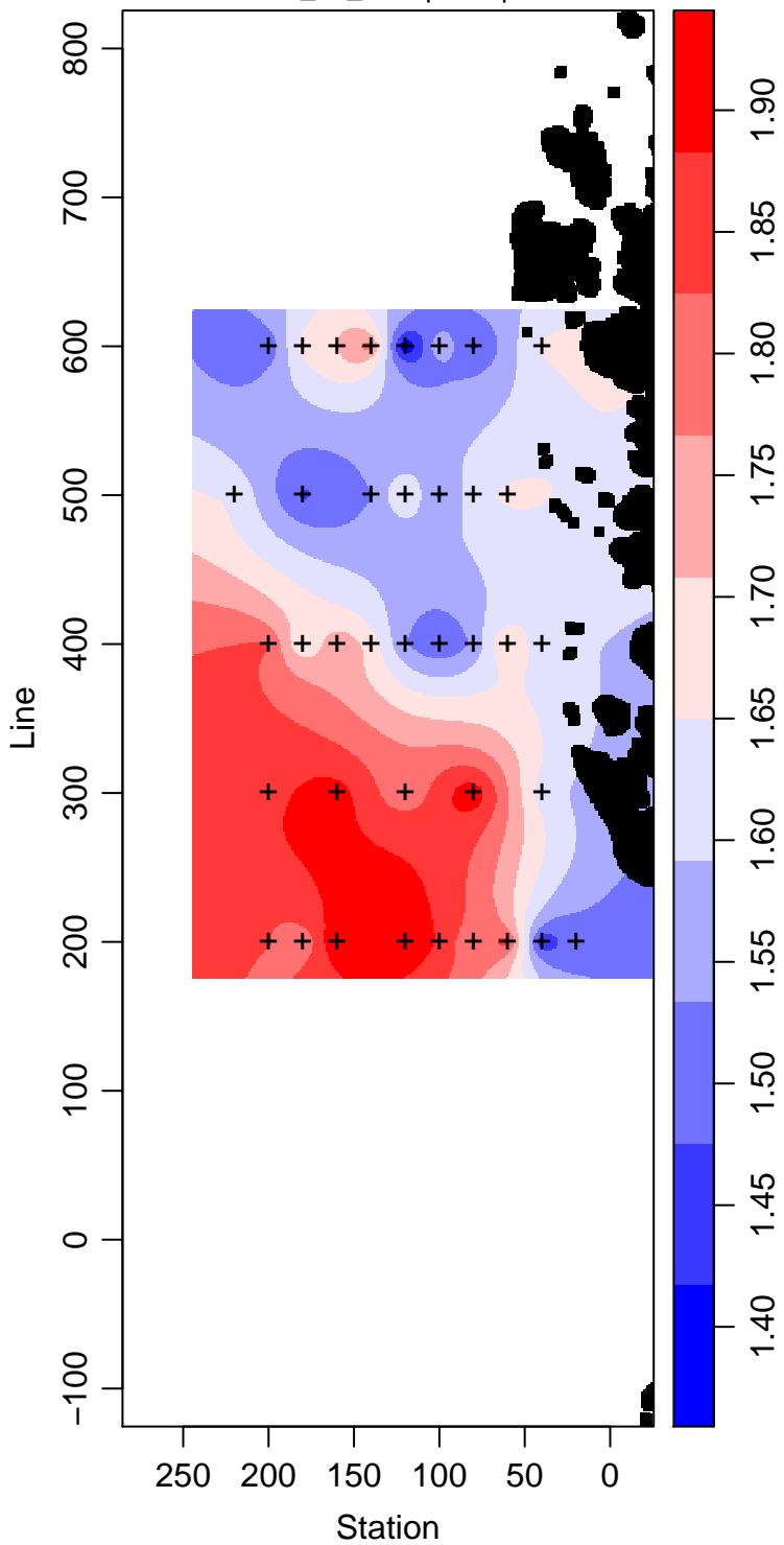
LMG01-01_55_Phosphate \mu\text{ mol L}^{-1}
