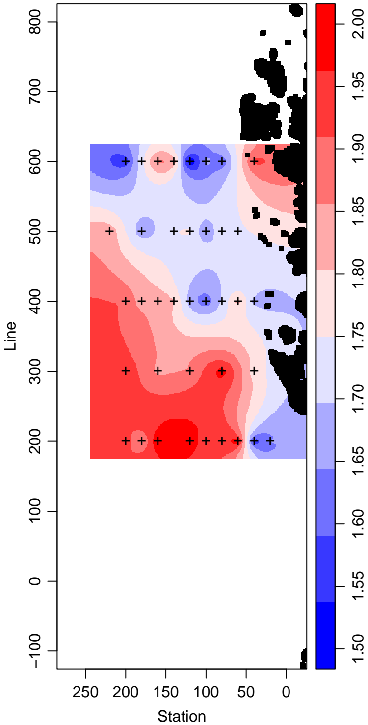
LMG01-01_65_Phosphate \mu\text{ mol L}^{-1}
