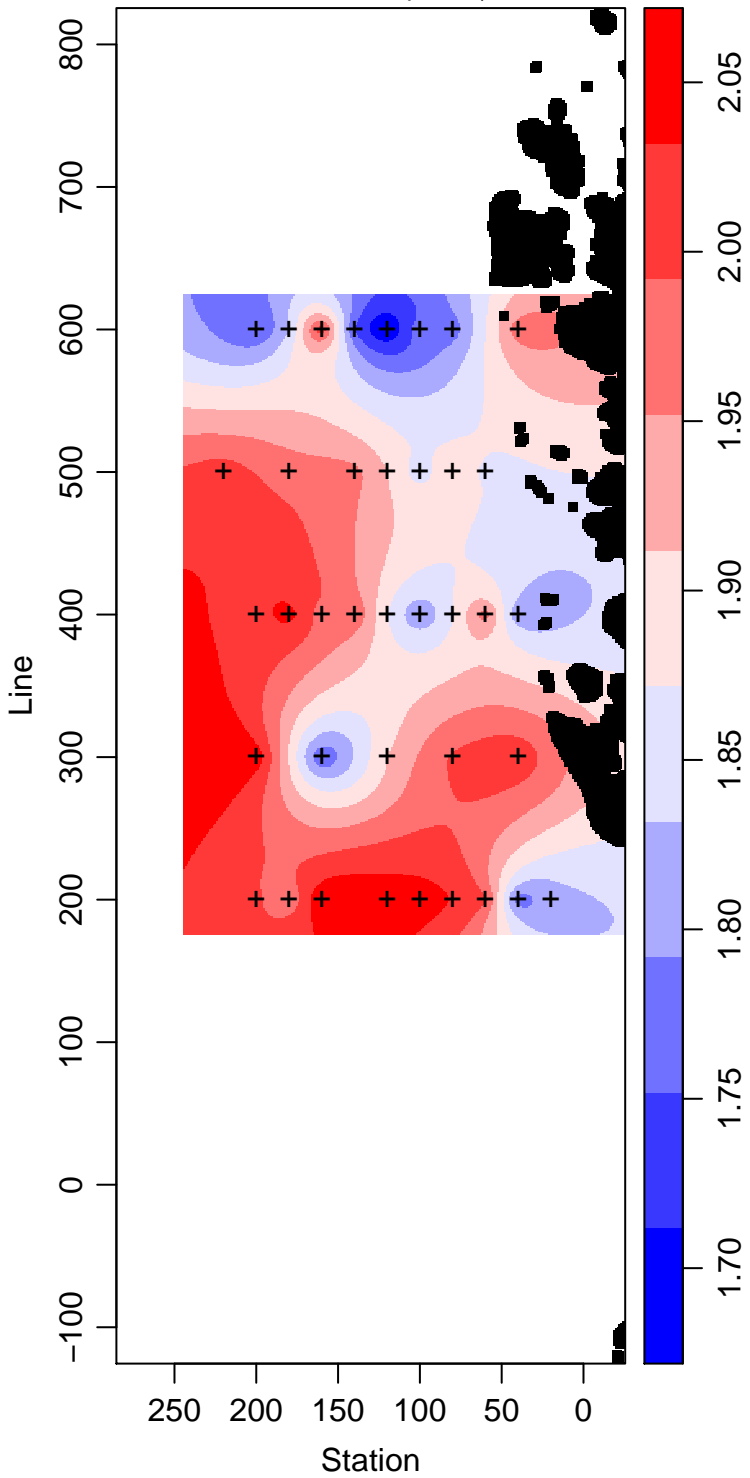
LMG01-01_80_Phosphate \mu\text{ mol L}^{-1}
