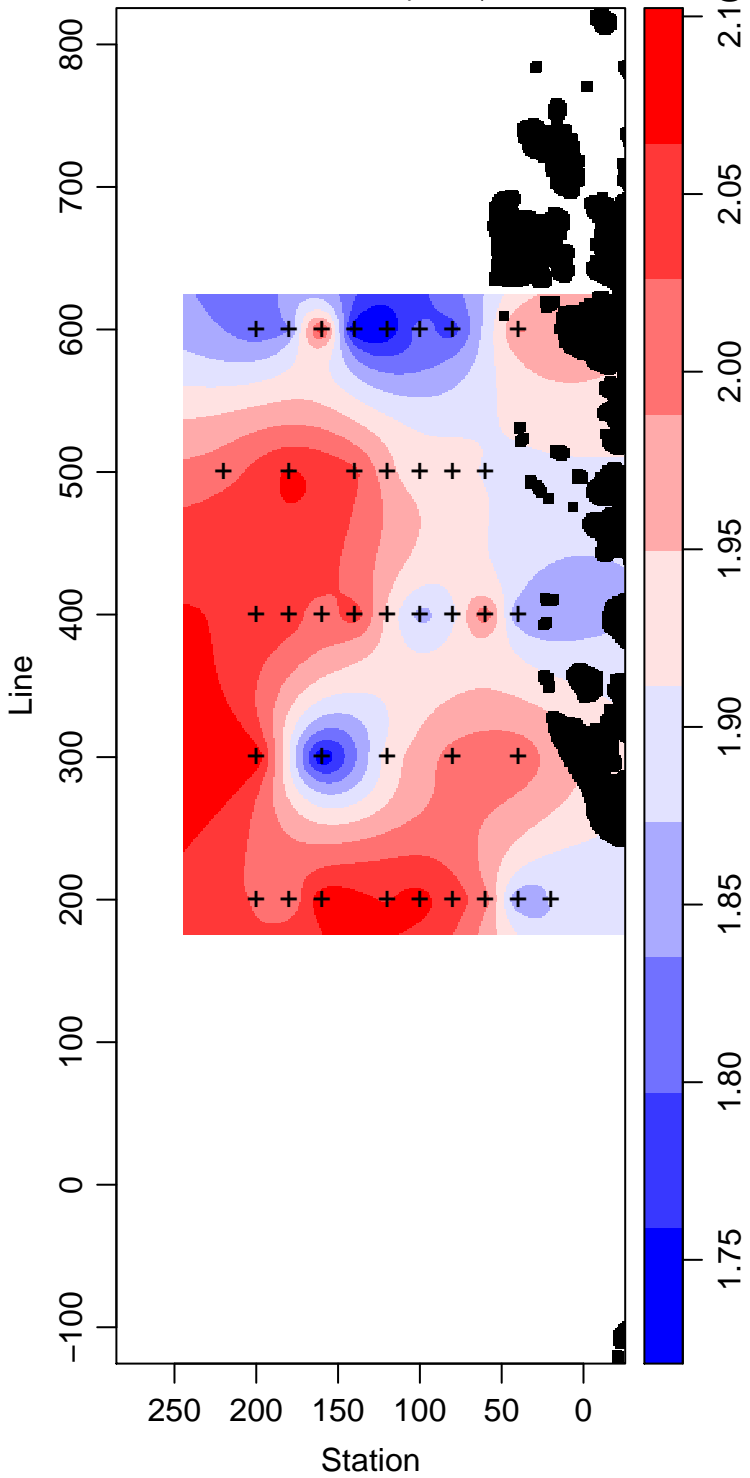
LMG01-01_85_Phosphate \mu\text{ mol L}^{-1}
