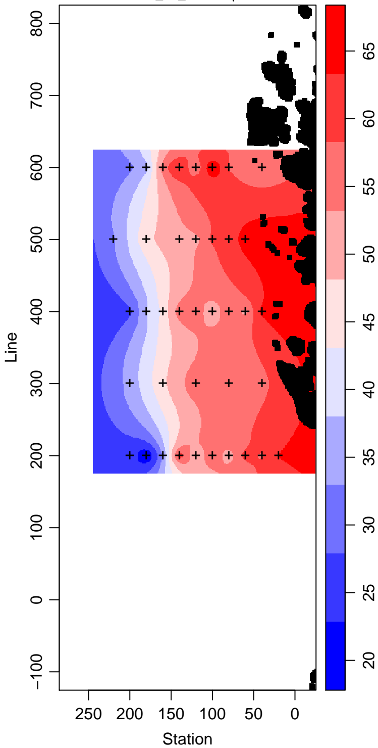
LMG01-01_15_Silicate \mu\text{ mol L}^{-1}
