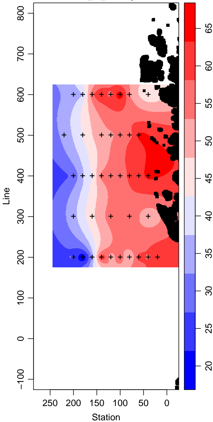
LMG01-01_20_Silicate \mu\text{ mol L}^{-1}
