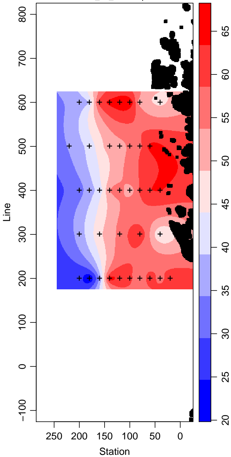
LMG01-01_25_Silicate \mu\text{ mol L}^{-1}
